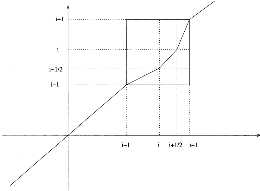
FIGURE 4. Graph of \tilde{G}_i = y_i y_{i+1}^{-1} , i \in \mathbb{Z}
