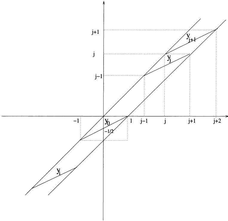
FIGURE 3. Graphs of y_i, i \in \mathbb{Z} . Note y_j y_i = y_i y_{j+1} when i < j .
