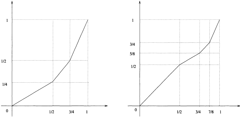
FIGURE 1. Graphs of generators A = x_0 and B = x_1
