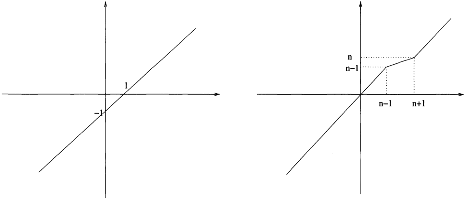
FIGURE 2. Graphs of generators \tilde{x}_0 and \tilde{x}_n , n \geq 1
