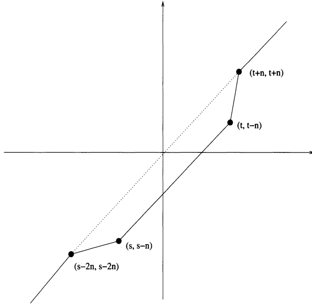
FIGURE 5. Graph of \tilde{h}
