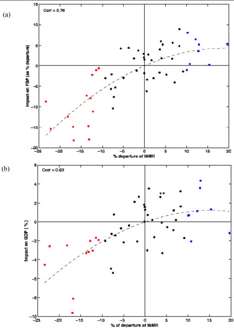
Figure 2. a) Variation of the impact on foodgrain production (IFGP) and b) Variation of the impact on GDP (IGDP) with the monsoon rainfall anomaly; drought and excess rainfall years are red and blue respectively.
